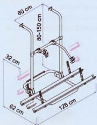
OMNI-BIKE plus 2 bikes
