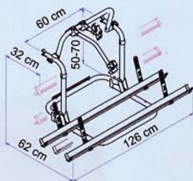
OMNI-BIKE plus 2 bikes short version
