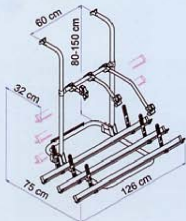
OMNI-BIKE plus 3 bikes
