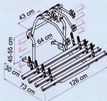
OMNI-BIKE plus 4 bikes short version
