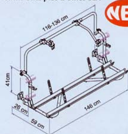
OMNI-BIKE plus 2 bikes SEA
