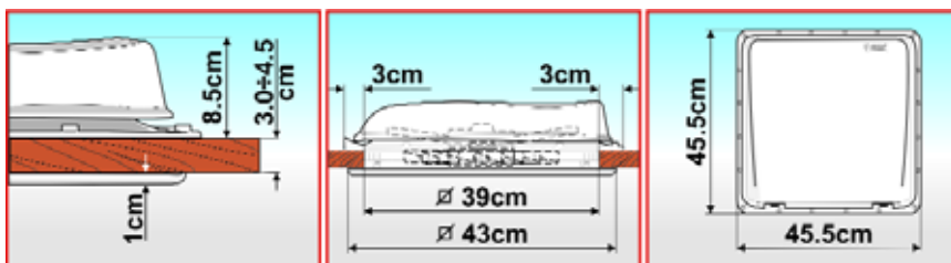
Turbo-Vent P3 Crystal
