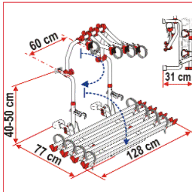
Carry-Bike Pro C with: 2 Rail Quick 128 Red, Bike-Block Pro 1 Red, Bike-Block Pro 3 Red
